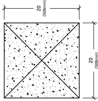
PLAN VIEW
