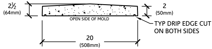
SECTION VIEW
