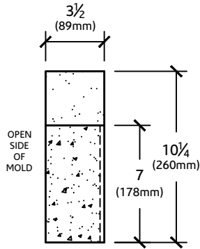
SECTION VIEW
