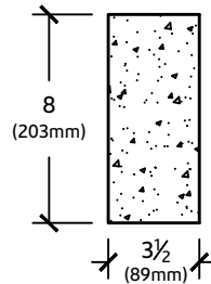
SECTION VIEW
