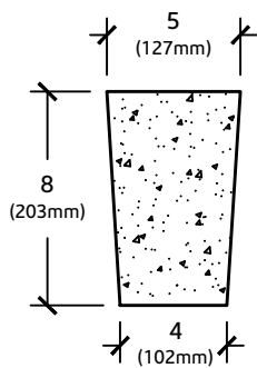
ELEVATION VIEW
