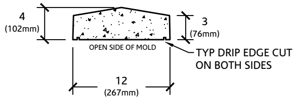
SECTION VIEW
