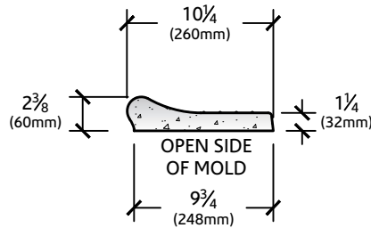
SECTION VIEW
