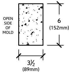
SECTION VIEW
