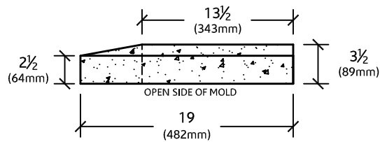
ELEVATION VIEW
