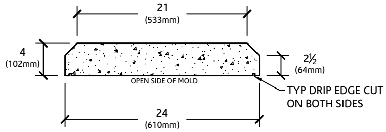
SECTION VIEW
