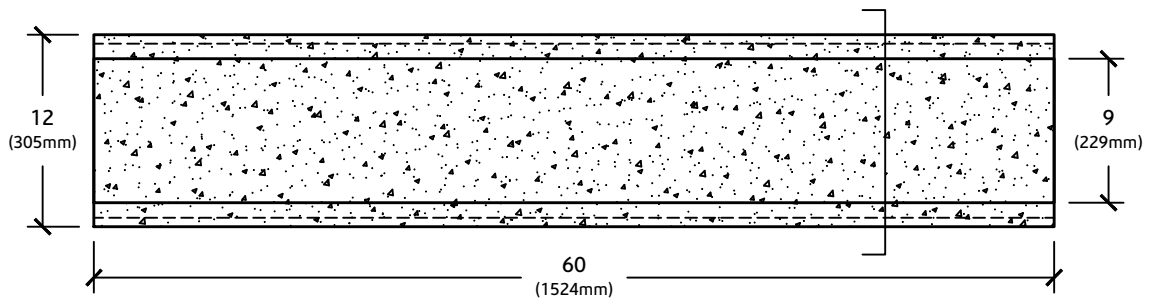
PLAN VIEW
