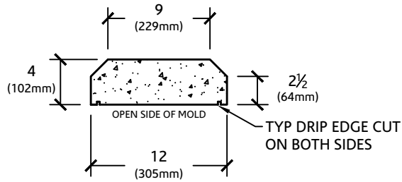
SECTION VIEW
