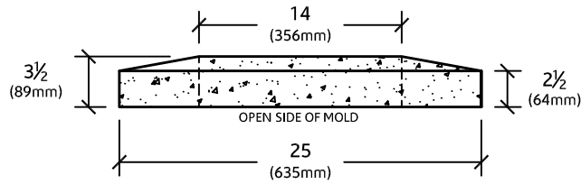
ELEVATION VIEW
