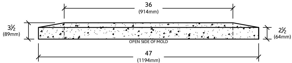
ELEVATION VIEW
