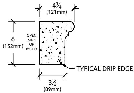
SECTION VIEW
