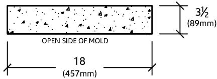
ELEVATION VIEW
