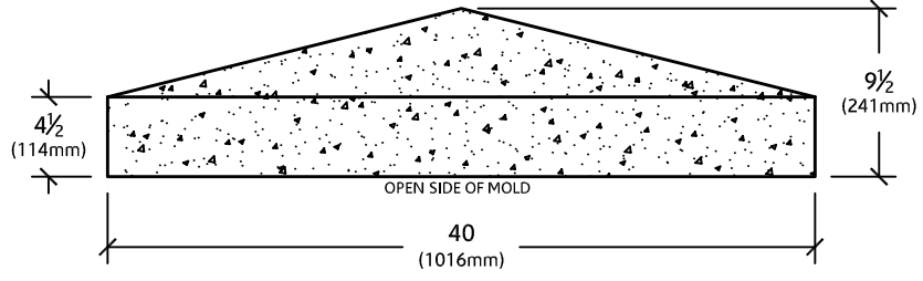
ELEVATION VIEW
