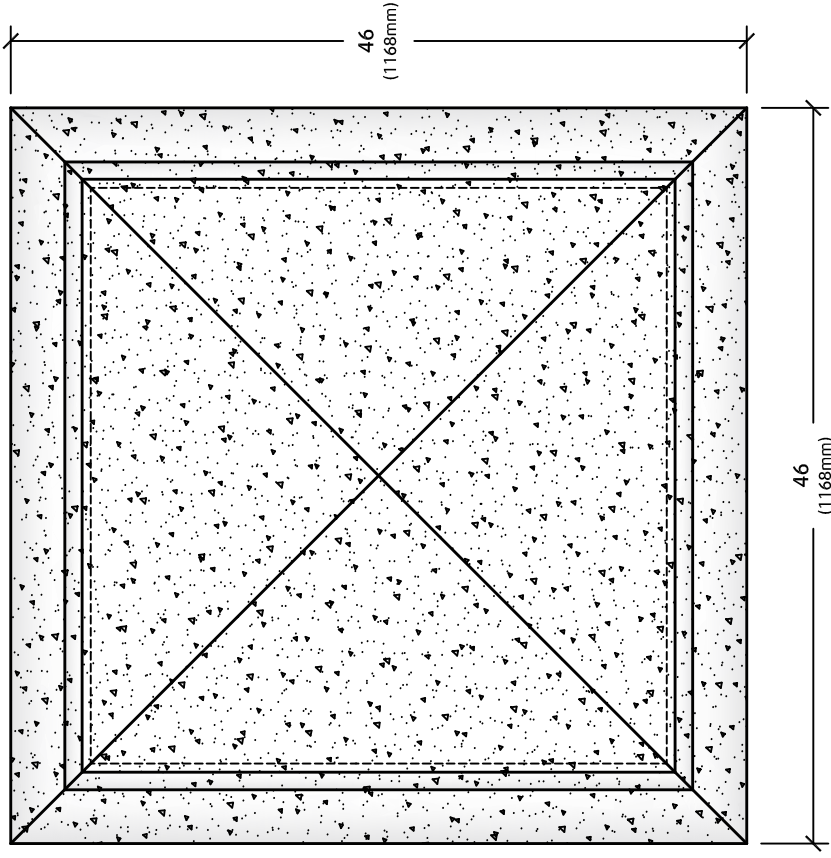
PLAN VIEW
