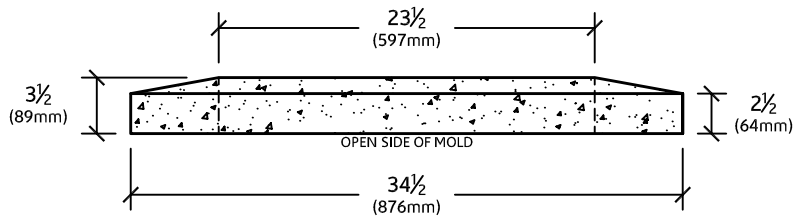
ELEVATION VIEW
