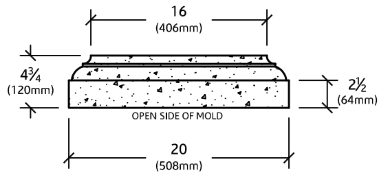
ELEVATION VIEW
