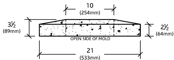
ELEVATION VIEW
