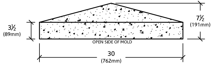
ELEVATION VIEW
