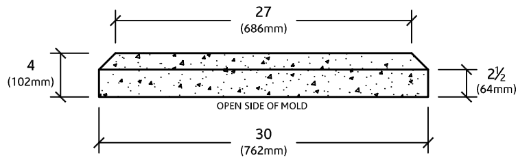
ELEVATION VIEW
