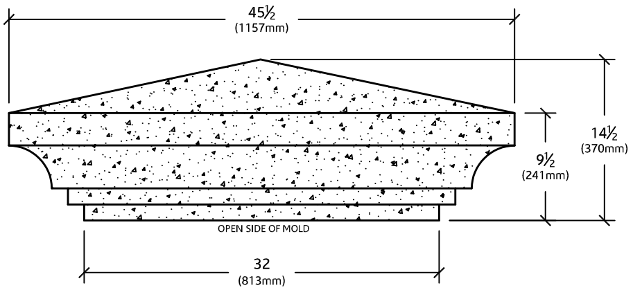
ELEVATION VIEW
