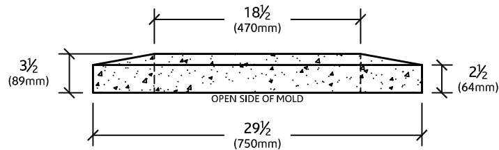
ELEVATION VIEW
