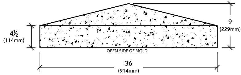
ELEVATION VIEW
