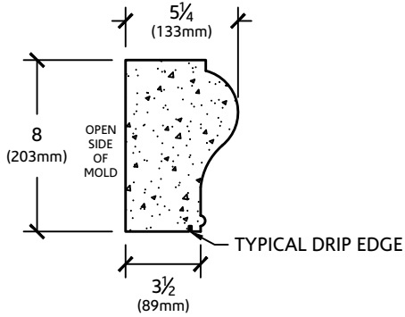
SECTION VIEW
