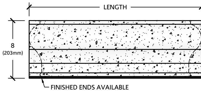
ELEVATION VIEW
