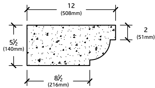
ELEVATION VIEW
