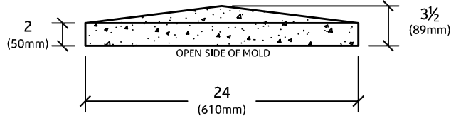
ELEVATION VIEW
