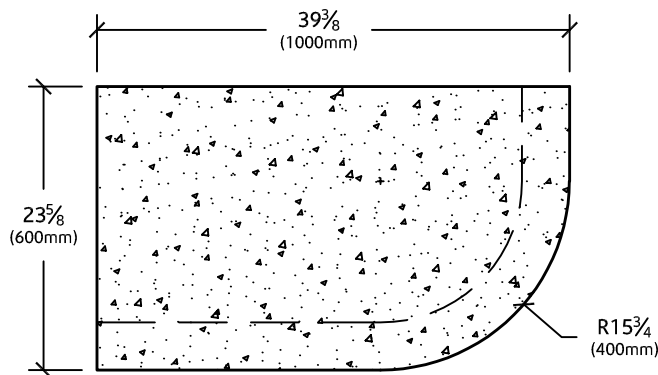
PLAN VIEW
