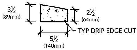
SECTION VIEW
