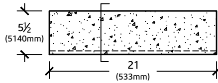
PLAN VIEW
