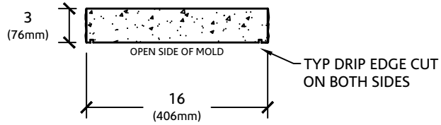
SECTION VIEW
