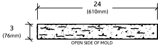
ELEVATION VIEW
