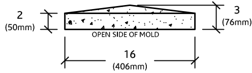
ELEVATION VIEW
