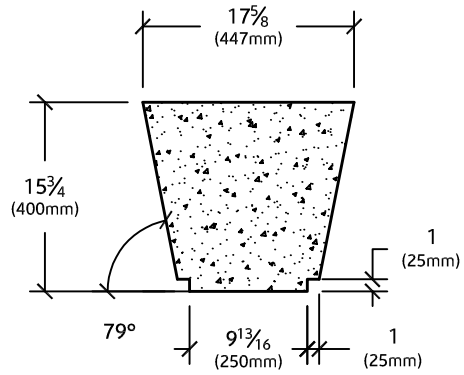
SECTION VIEW
