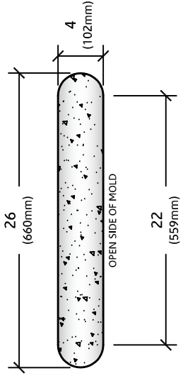
ELEVATION VIEW
