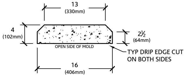
SECTION VIEW
