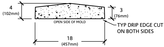
SECTION VIEW
