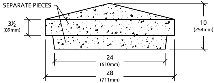
ELEVATION VIEW
