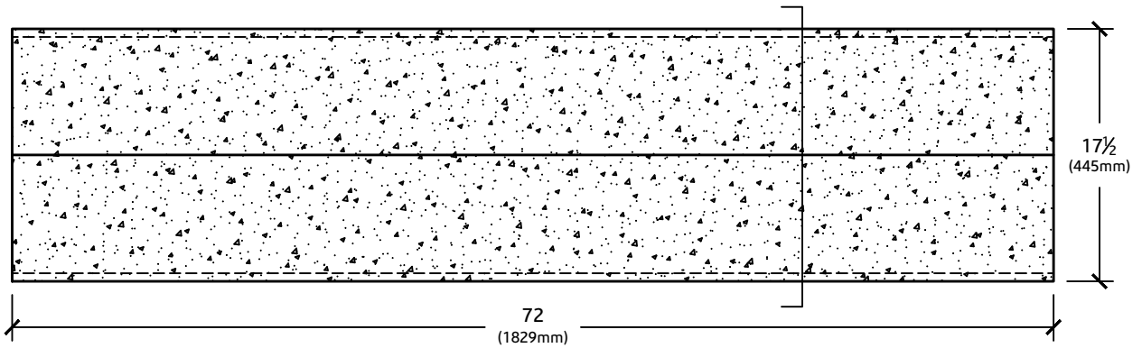
PLAN VIEW
