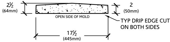
SECTION VIEW
