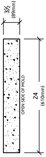
ELEVATION VIEW
