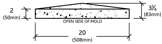
ELEVATION VIEW
