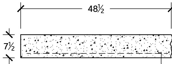
ELEVATION VIEW
