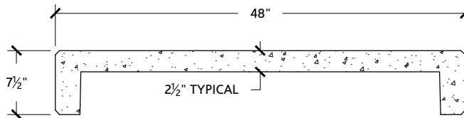
SECTION VIEW
