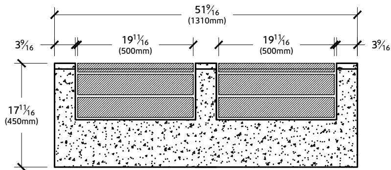
ELEVATION VIEW
