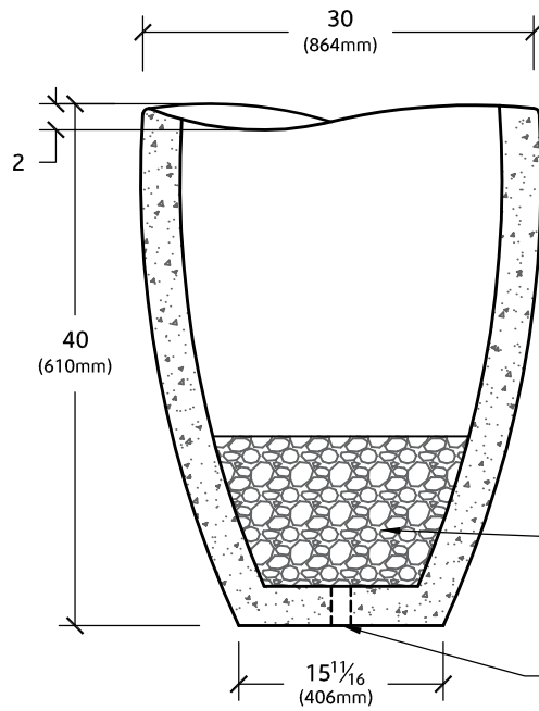
SECTION VIEW
