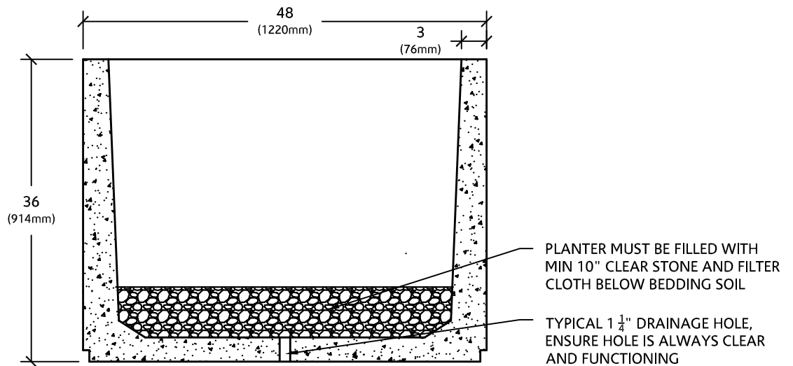
SECTION VIEW
