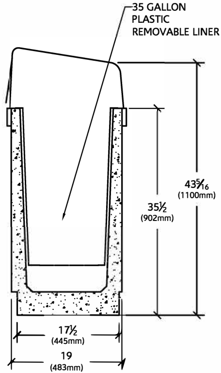
SECTION VIEW
