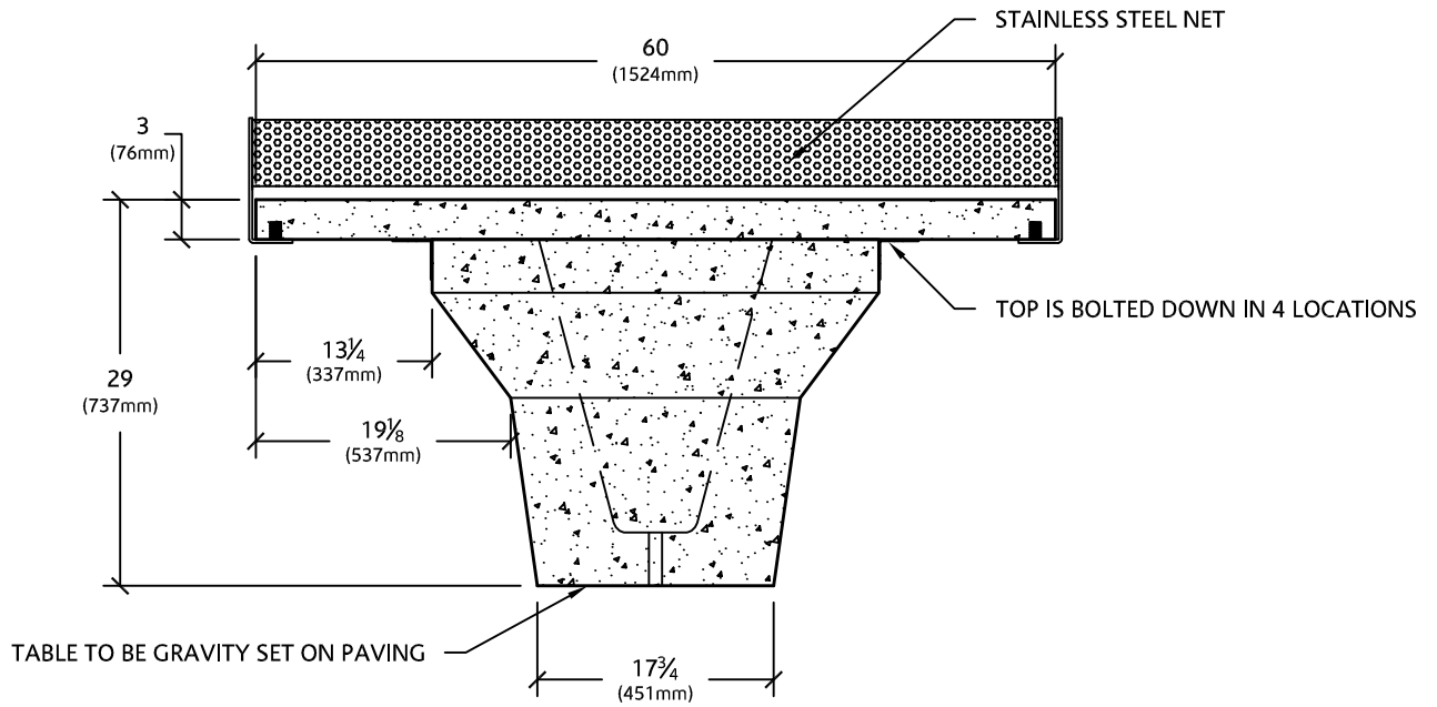
END VIEW
