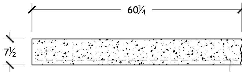
ELEVATION VIEW
