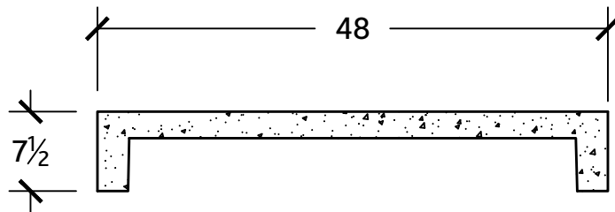
SECTION VIEW
