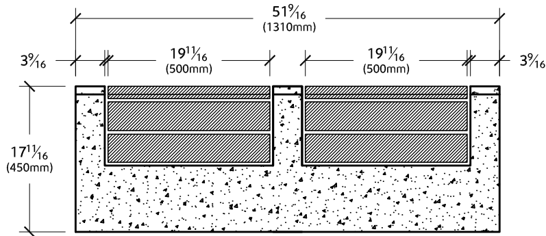
ELEVATION VIEW
