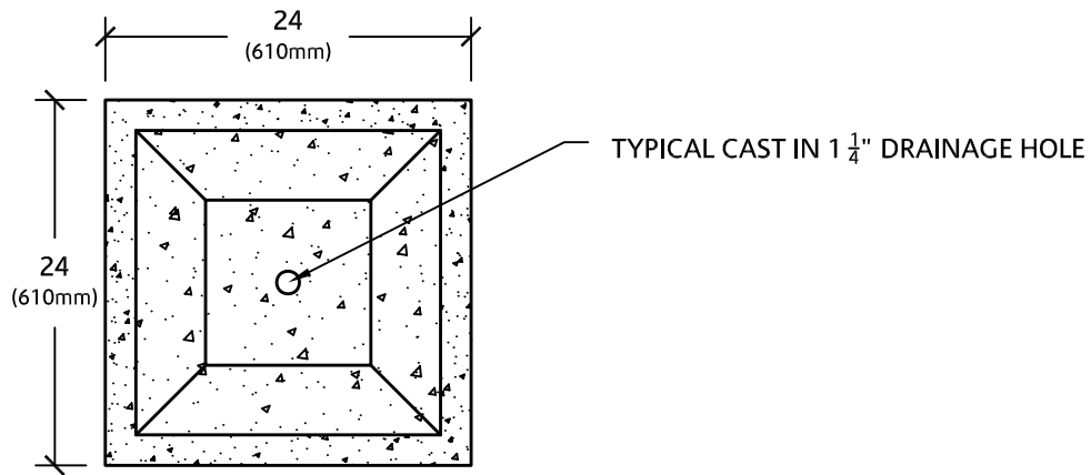
PLAN VIEW
