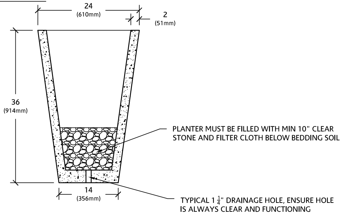
SECTION VIEW
